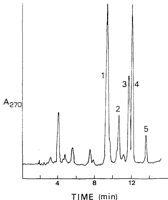
Figure 1. HPLC separation of flavonoid glycosides and phenolic acids of a methanol extract of Spartan apple peel: (1) quercetin glucoside and quercetin galactoside; (2) quercetin xyloside; (3) quercetin rhamnoside; (4) quercetin arabinoside; (5) phlorizin. Conditions: column, radial pak RP (C 18 ); solvent program, 25–50% THF in 0.1% aqueous TFA over 20 min at a flow rate of 2.0 mL/min with detection at 270 nm. Rutin was responsible for the peak at 7.5 min.
